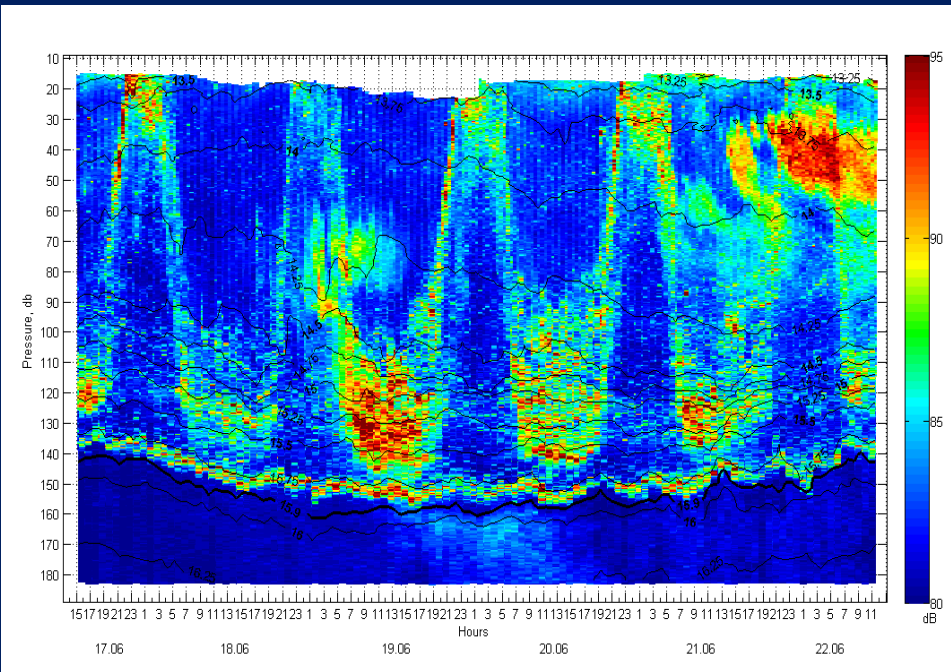
Acoustic backscatter signal (2 MHz). 17-22 June 2011
